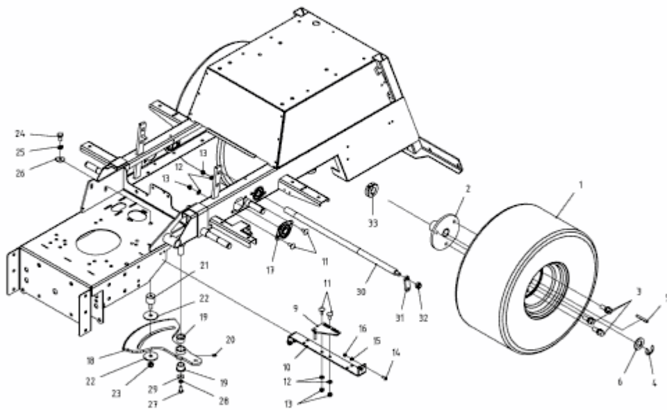
54A1F2Q-603 - 2200 RD - Blatt 6
