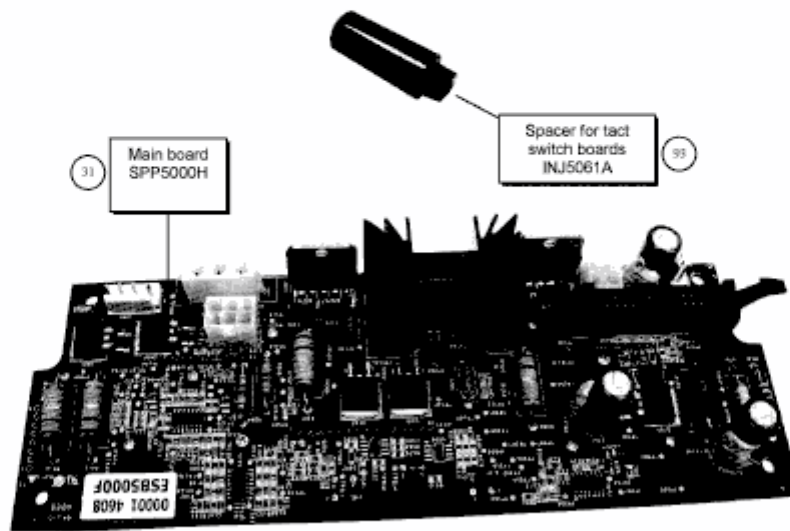
Main Board Top View
