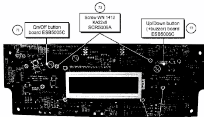
Main Board Top View
