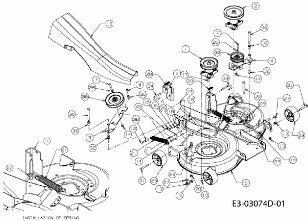
INSTALLATION OF SPRING
