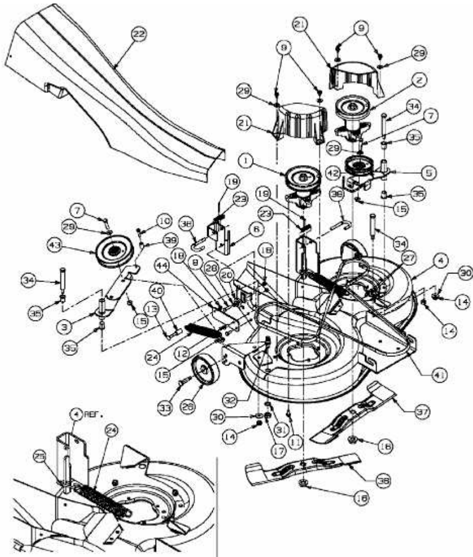
INSTALLATION OF SPRING Feder-Montage
