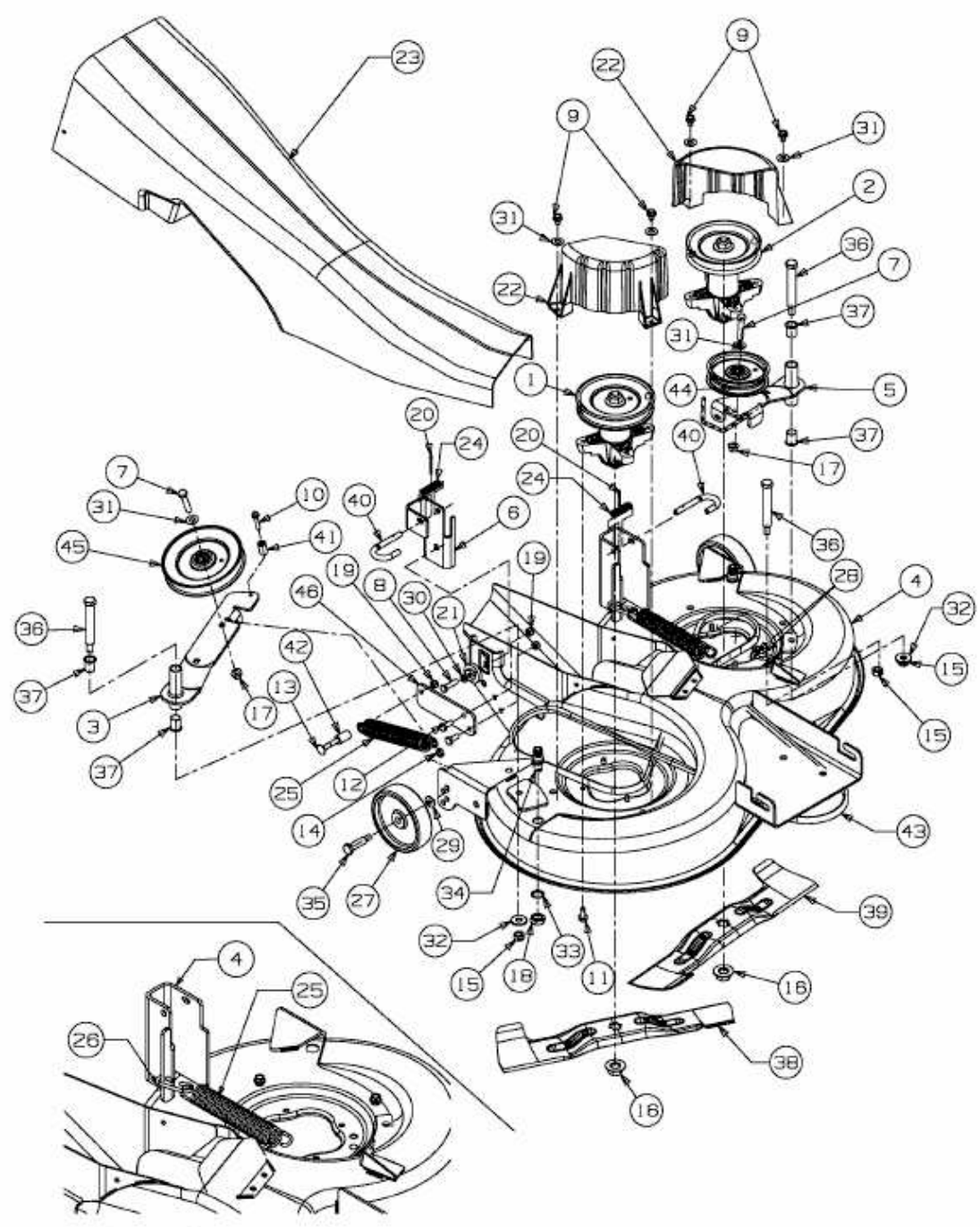
Installation of spring / Federmontage
