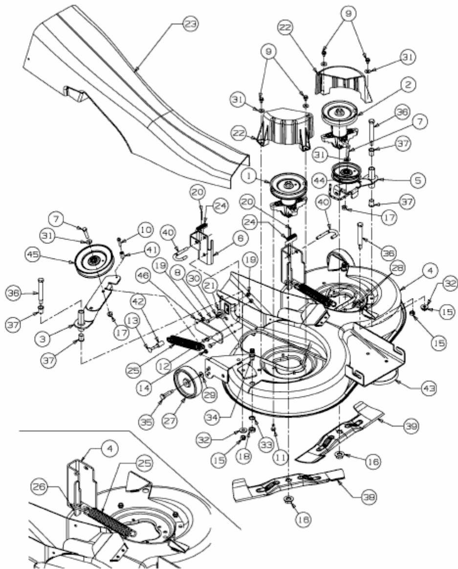
Installation of spring / Federmontage
