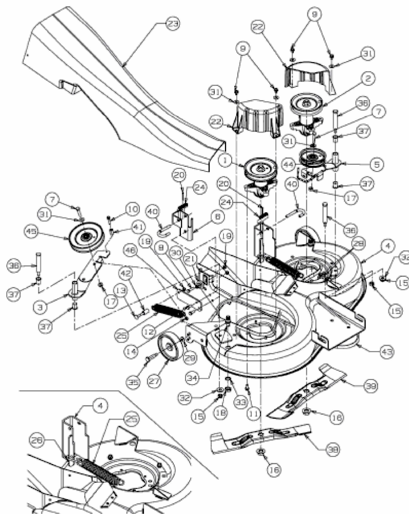
Installation of spring / Federmontage
