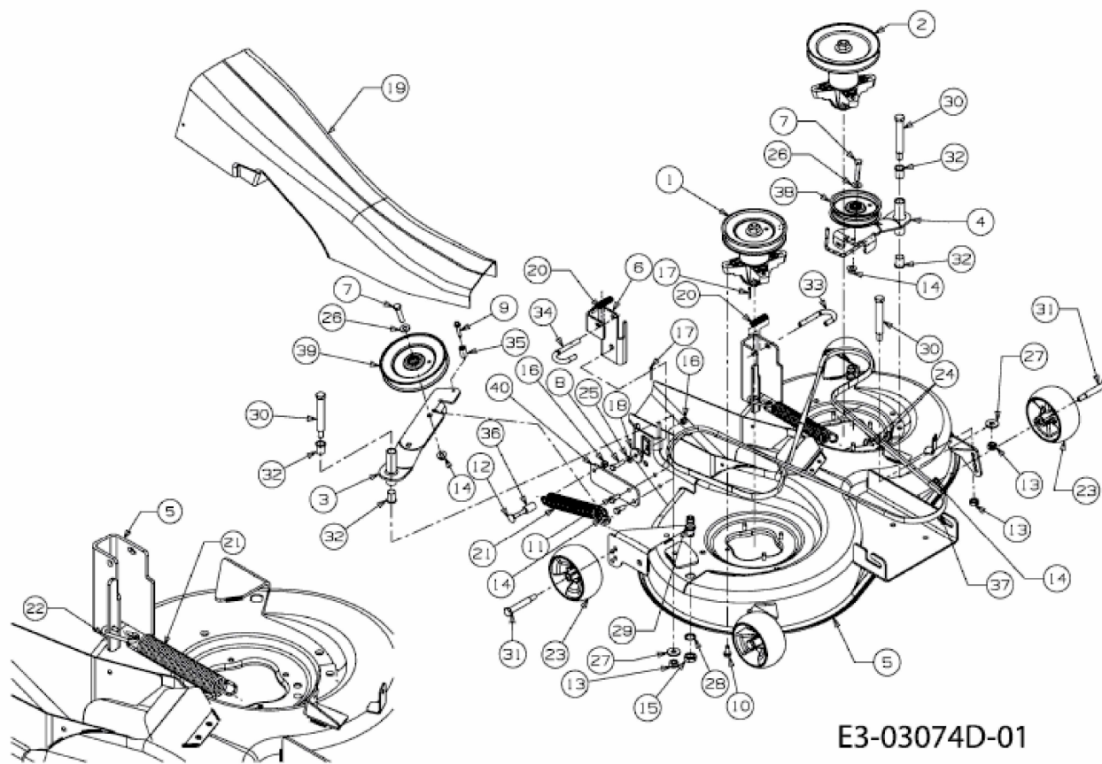
INSTALLATION OF SPRING
