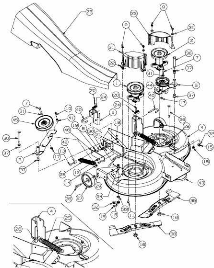
Installation of spring / Federmontage
