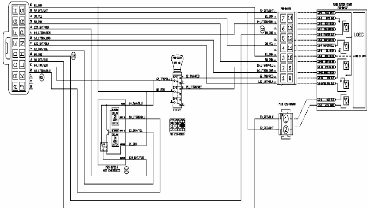
MAIN HARNESS CONNECTION 1 HTO 729-88152
