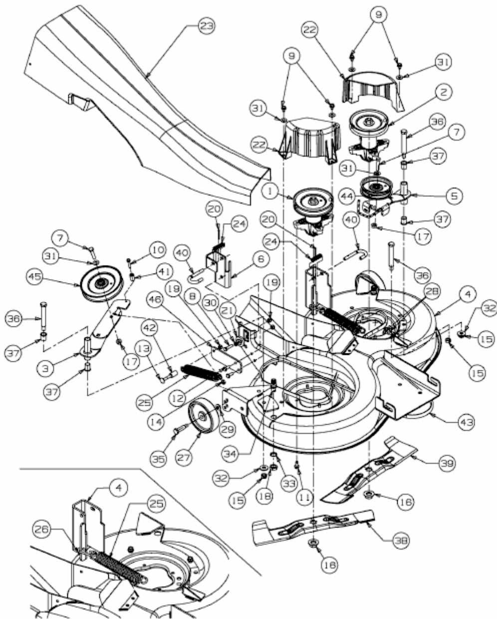
Installation of spring / Federmontage
