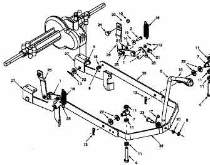
Deck Hanger Link
