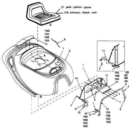
Hood Assembly
