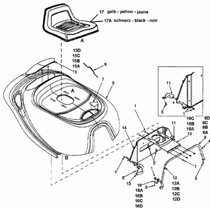
Hood Assembly
