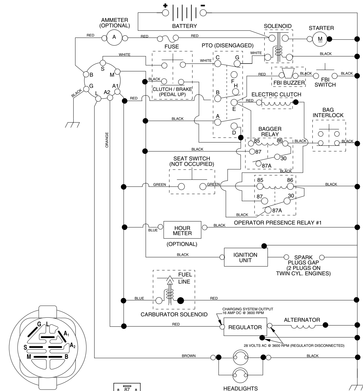
IGNITION SWITCH
